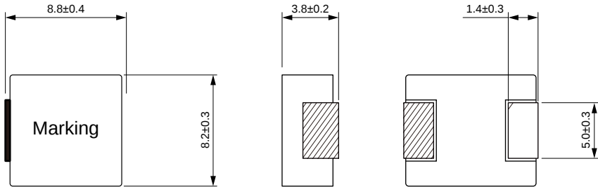
Dimensions: [mm]
