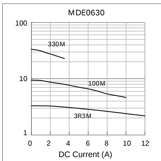
Inductance vs DC Current Characteristics:
