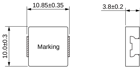
Dimensions: [mm]
